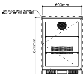
Front elevation
