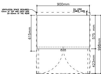
Floor plan
